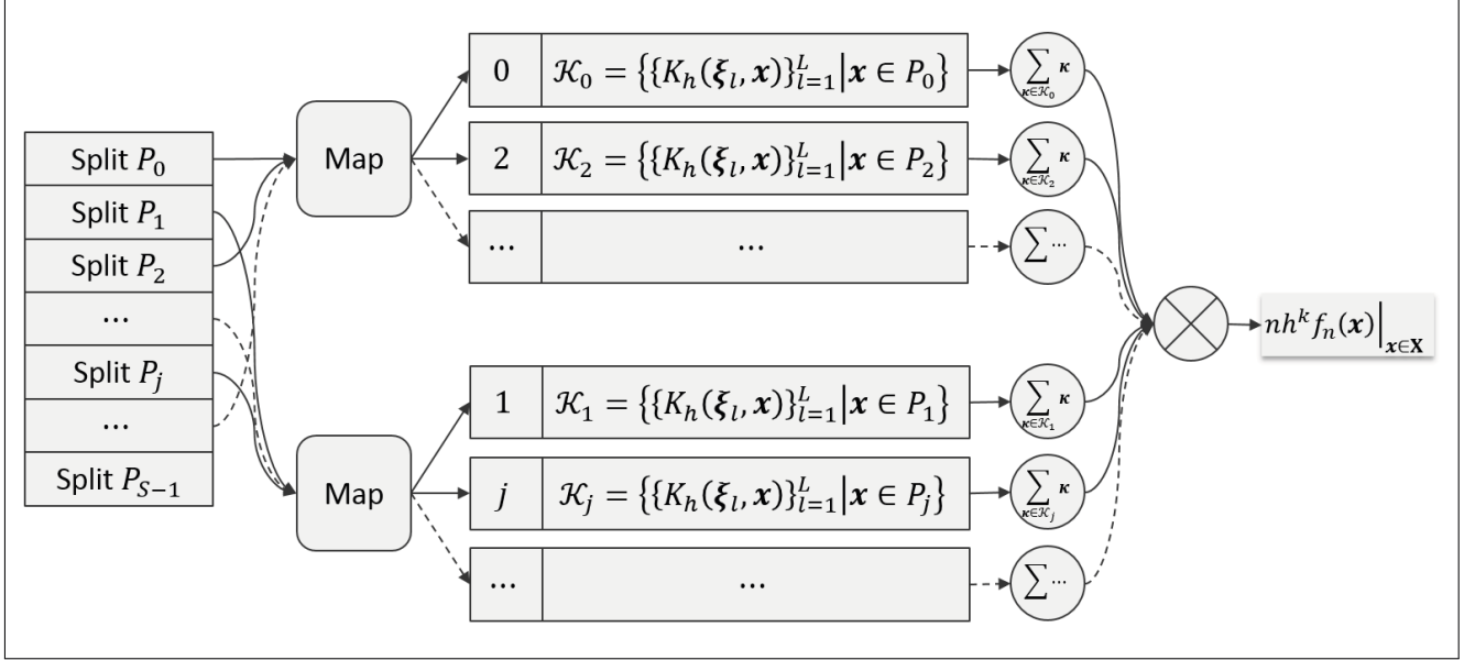
Figure 2. Implementation of the KDE with MapReduce logic. The leftmost block shows the the input data relative to a single port, which is organized in partitions and stored on a DFS or a distributed database. Taking advantage of its linearity, the computation of the KDE can be distributed among multiple nodes, each of which performs an expansion of the input partition with the Gaussian kernel.
