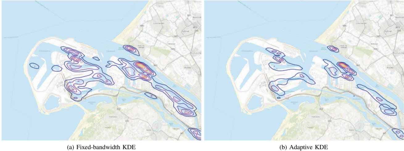
Figure 3. Comparison of fixed and adaptive bandwidth kernel density estimates computed in the Rotterdam port area. The fixed-bandwidth version (a) produces a smoother result, but is unable to deal satisfactorily with the low-density regions. The adaptive KDE (b) has a higher computational cost than the fixed KDE, but it produces a spikier , and consequently narrower, estimate on low-density regions. Both the estimates have been computed on the available data collected by MarineTraffic from January to March 2015, having selected only those ships whose speed reported by the AIS was not exceeding the fixed threshold of 1 kn.
