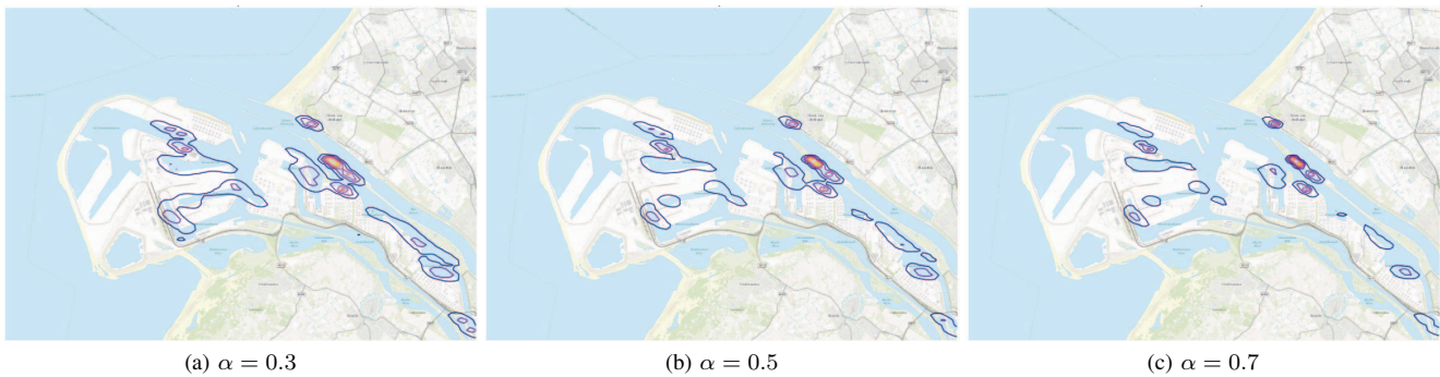
Figure 4. Effect of the sensitivity \alpha on the resulting PDF estimated with the adaptive bandwidth approach. The three panels refer to three different sensitivity levels, namely \alpha = 0.3 (a), \alpha = 0.5 (b) and \alpha = 0.7 (c). Smaller values of the sensitivity parameter \alpha produce results that are more similar to the fixed-bandwidth KDE, while spikier density functions are created with higher values of \alpha , but they are inevitable more fragmented.
