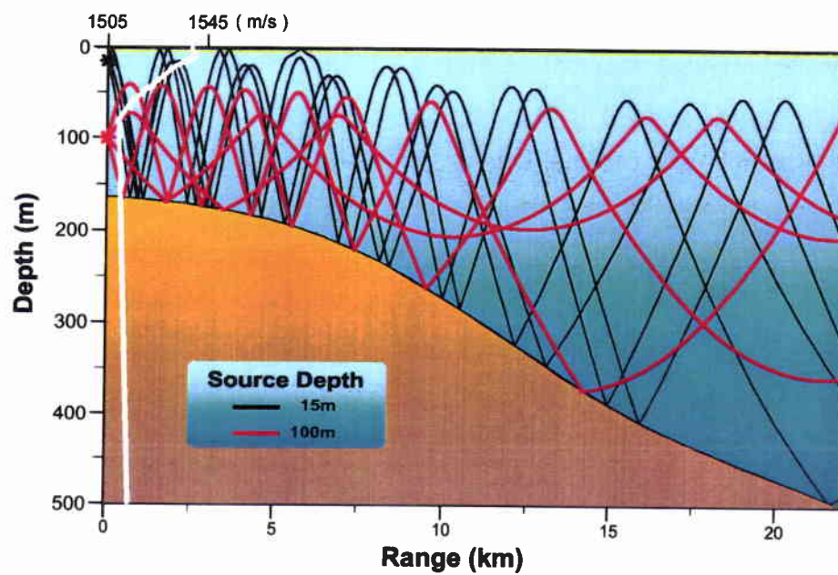
Figure 32 Track B – downslope: Ray diagrams for two different source depths.
