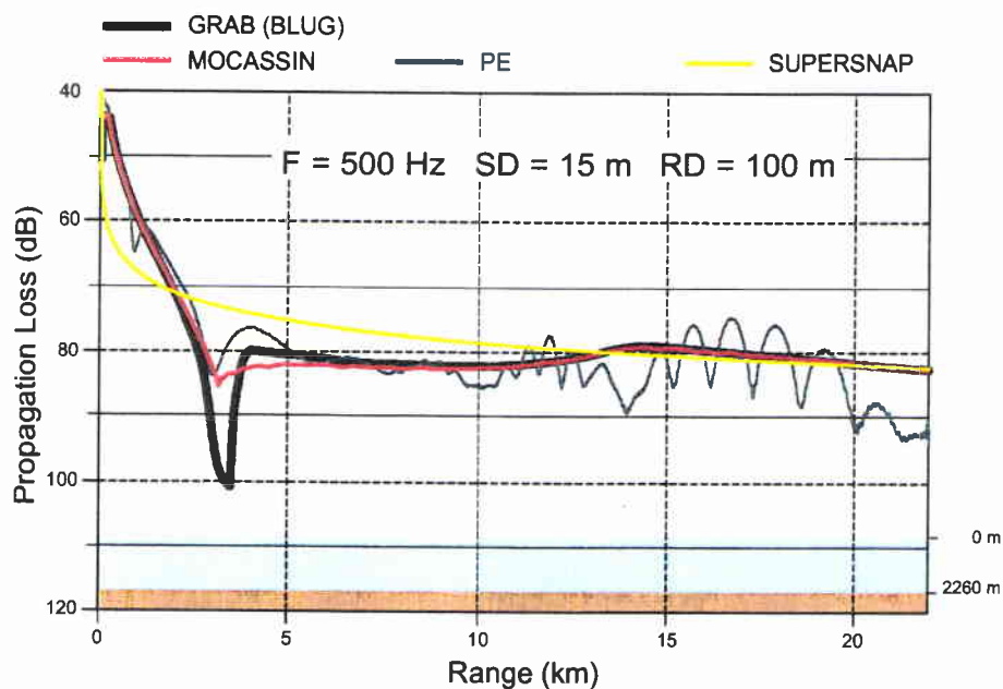
Figure A3 Track A – flat: Inter-model comparison at 500 Hz for source at 15 m and receiver at 100 m.
