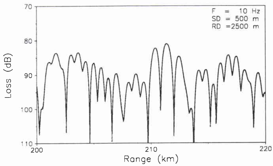
Figure 5.2: Transmission loss for the PEKERIS problem.
