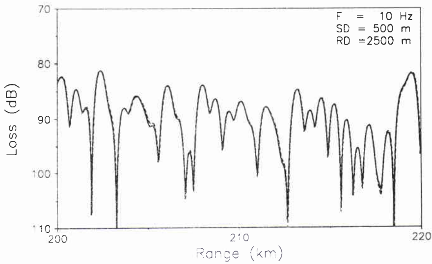
Figure 5.12: Transmission loss for the ELSEED problem.
