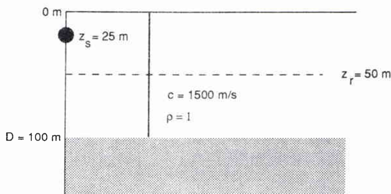
Figure 2.2: Schematic of the isovelocity problem.
