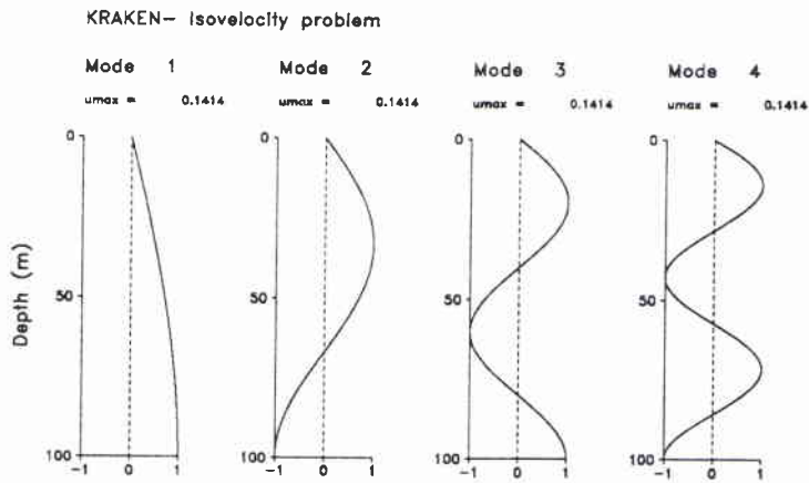
Figure 2.4: Selected modes of the isovelocity problem.
