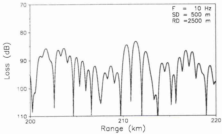
Figure 5.14: Transmission loss for the ATTEN problem.
