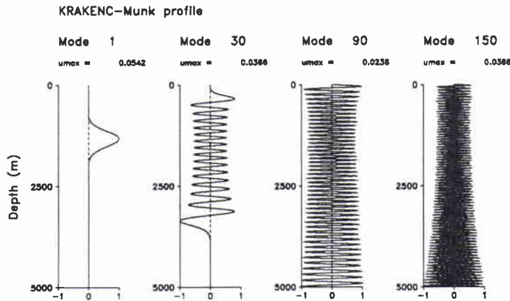
Figure 2.11: Selected modes for the deep-water problem.
