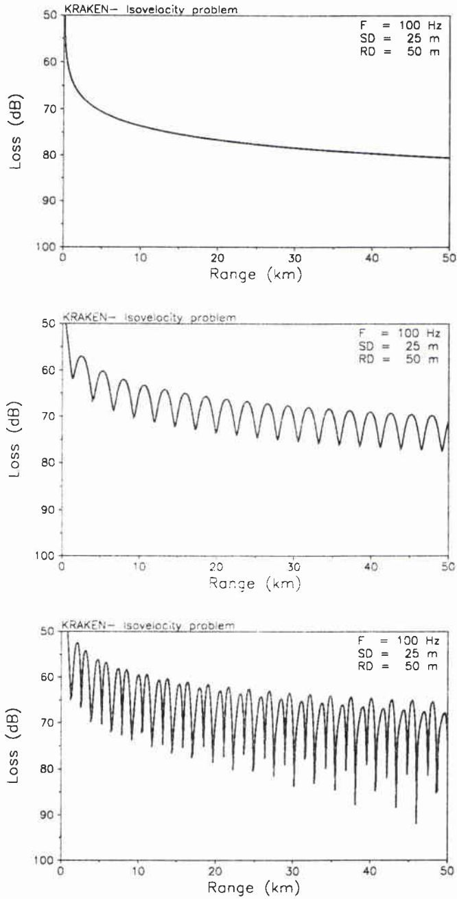
Figure 2.5: Transmission loss for the isovelocity problem using (a) 1 mode, (b) 2 modes and (c) 3 modes.
