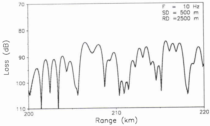
Figure 5.6: Transmission loss for the DOUBLE problem.
