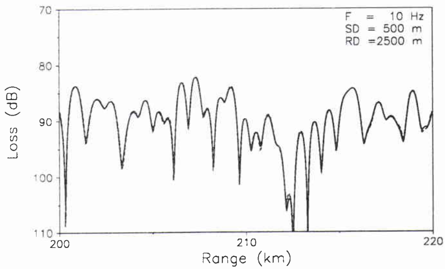
Figure 5.10: Transmission loss for the FLUSED problem.
