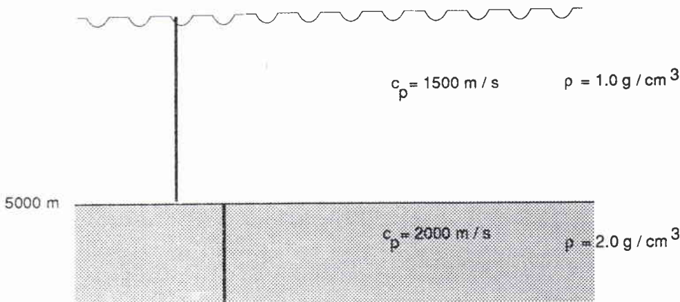
Figure 5.3: Schematic of the TWERSKY problem.
