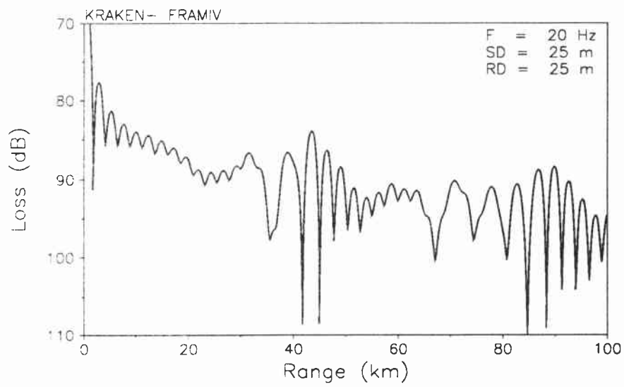
Figure 4.8: Sample output of PLOTTLR: transmission loss vs. range for the Arctic problem.
