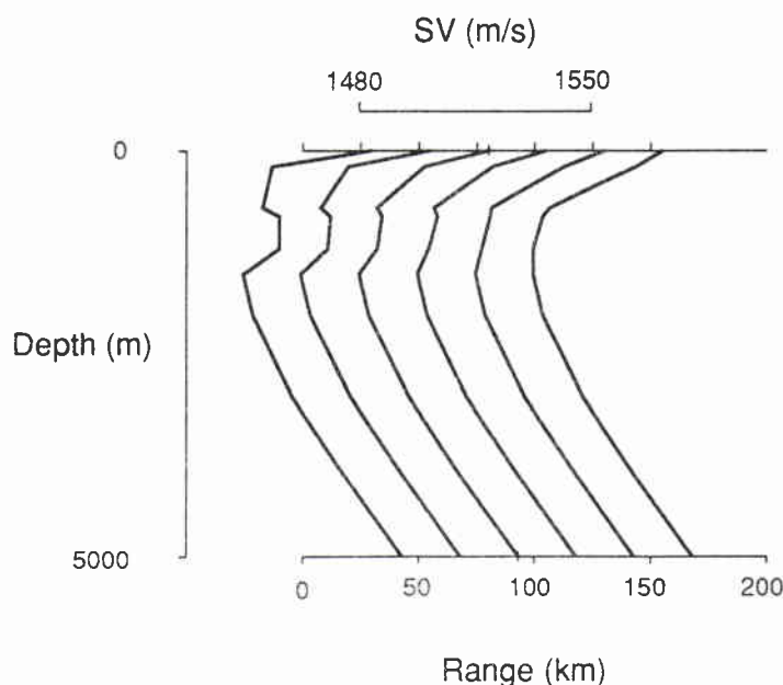
Figure 2.14: Sound speed profiles taken through the eddy.
