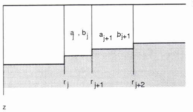
Figure 2.13: Segmentation for coupled mode formulation.
