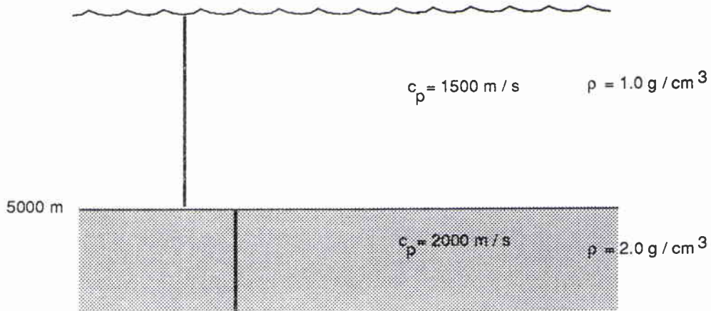
Figure 5.1: Schematic of the PEKERIS problem.
