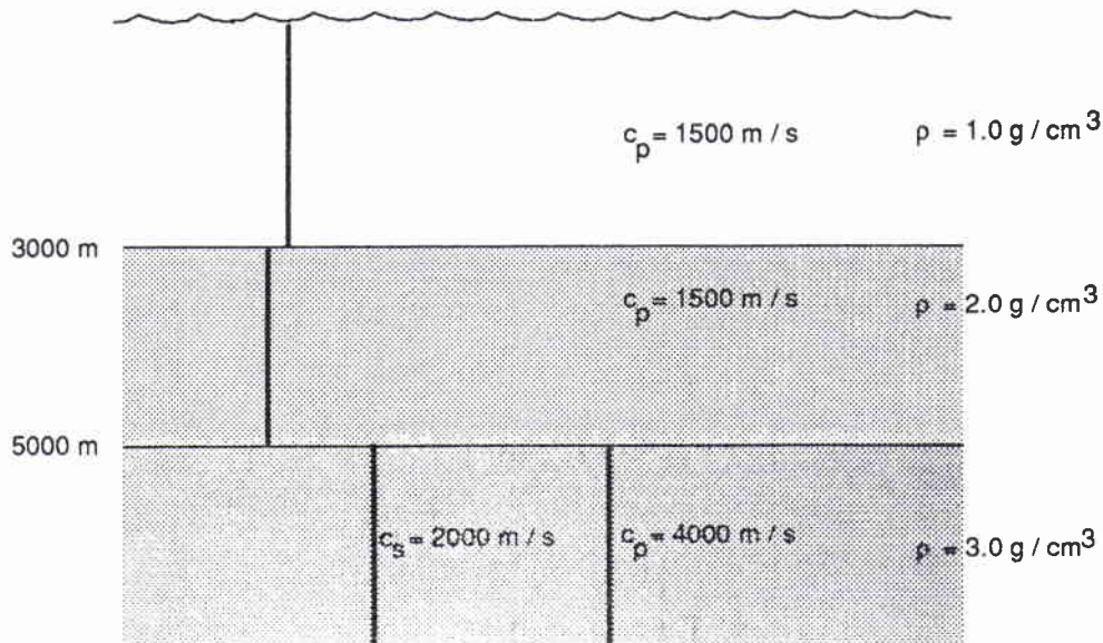
Figure 5.15: Schematic of the NORMAL problem.
