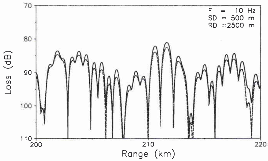
Figure 5.18: Transmission loss for the ICE problem.
