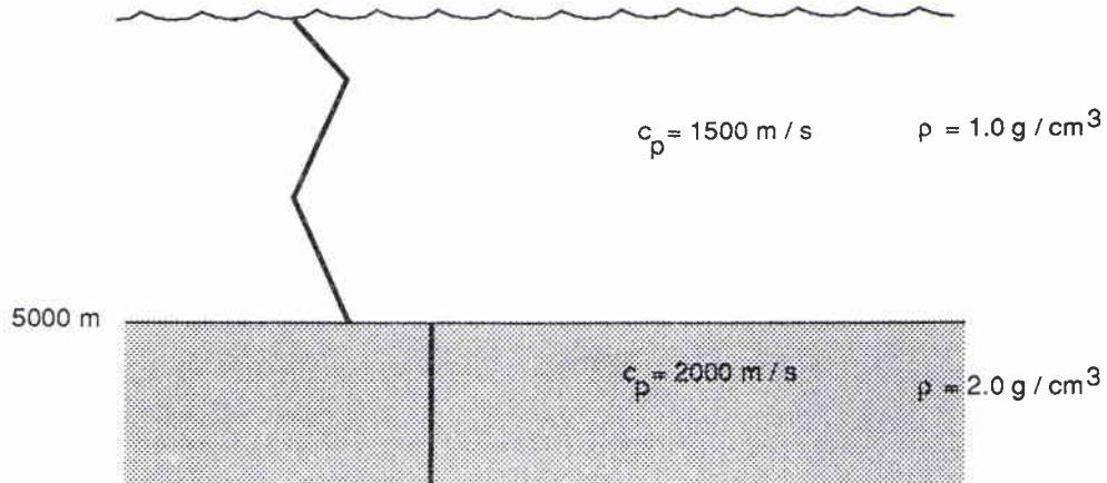
Figure 5.5: Schematic of the DOUBLE problem.
