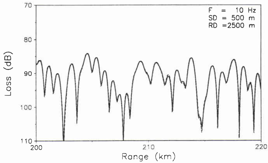
Figure 5.16: Transmission loss for the NORMAL problem.
